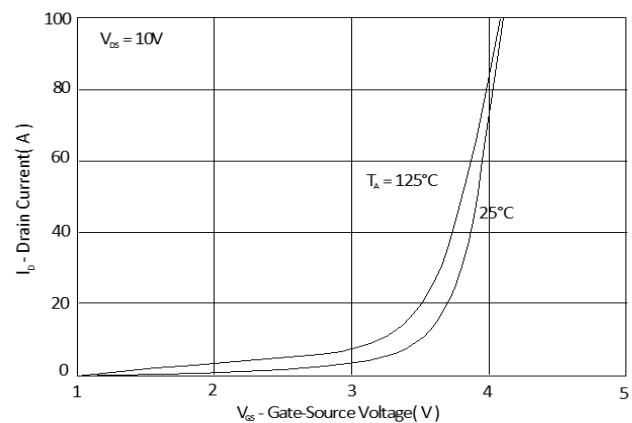
Fig.6 Transfer Characteristics
