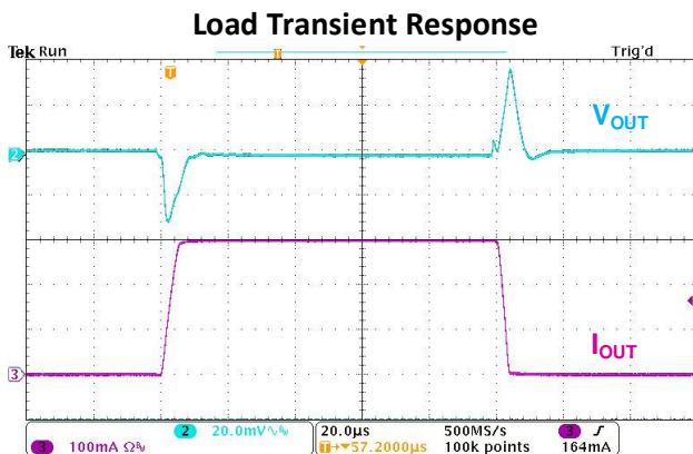
V_{IN}=4.3V , V_{OUT}=3.3V , C_{IN}=C_{OUT}=1\mu F
